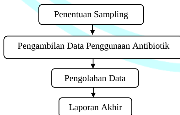
Gambar 3.1 Alur Penelitian
