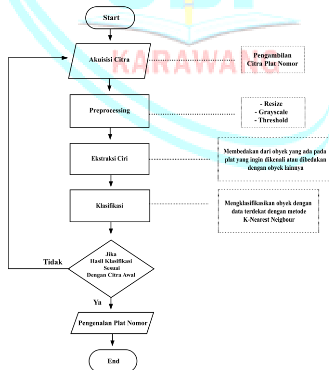
Gambar 3.2 Flowchart Tahapan Penelitian
